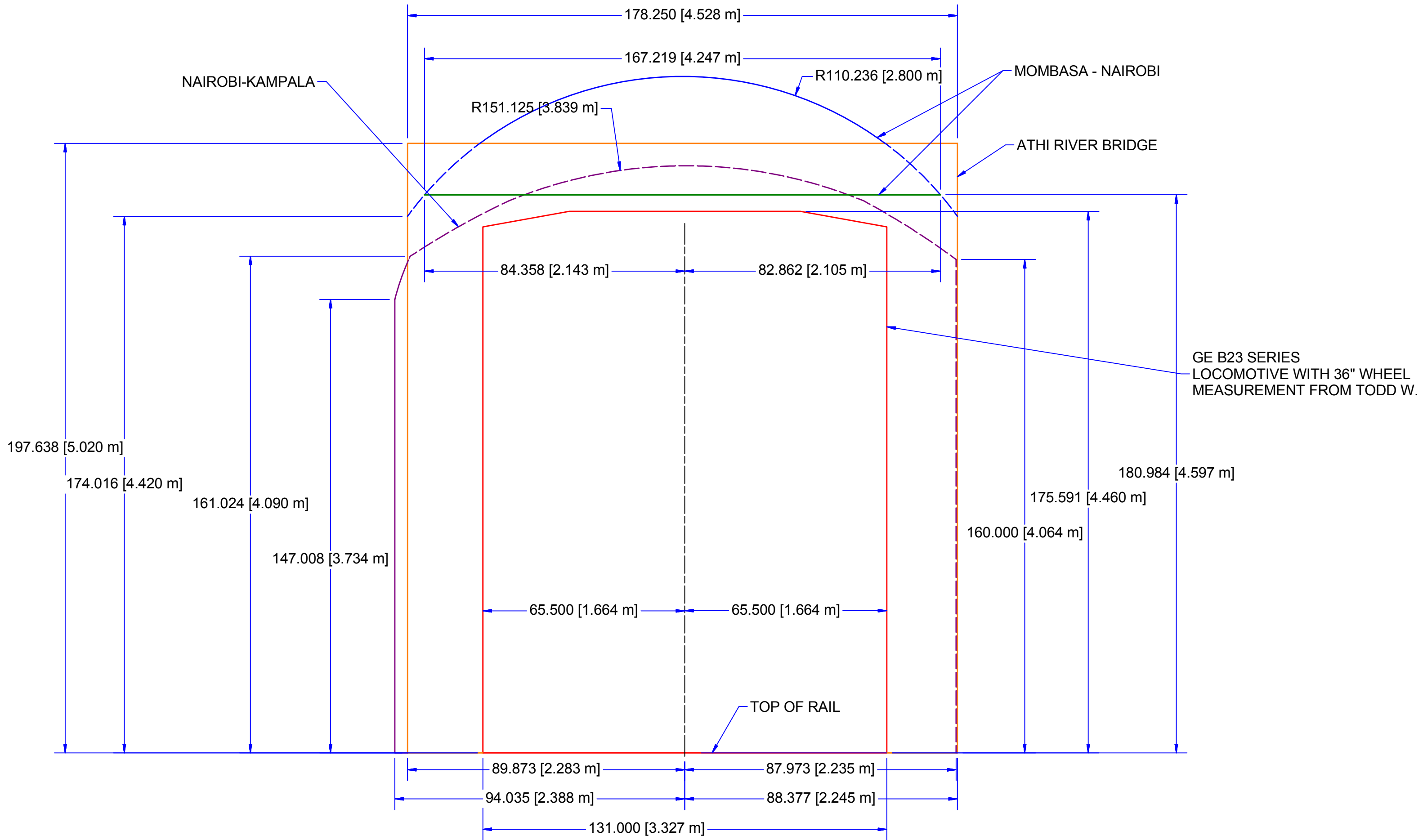
LOADING DIAGRAM
